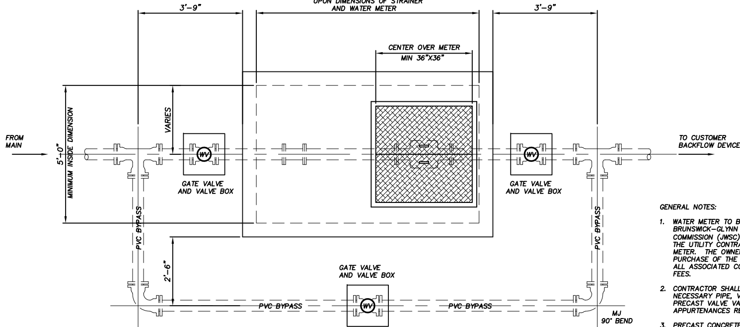
TOP PLAN
