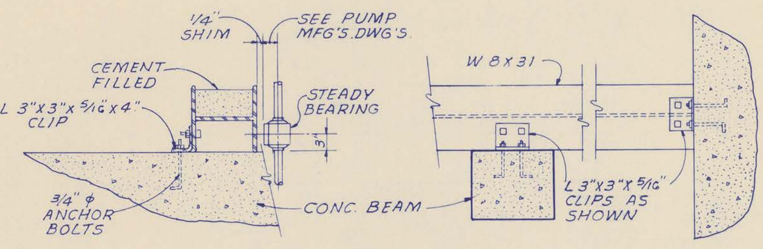
STEADY BEARING SUPPORT N.T.S.
