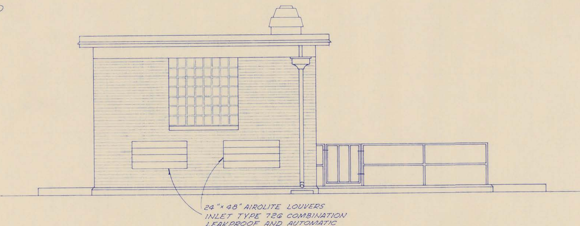
RIGHT SIDE ELEVATION 1/4"=1'-0"
