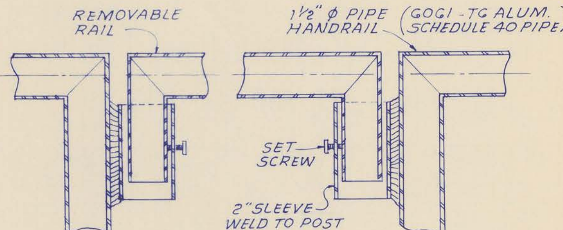
REMOVABLE SECTION 1 1/2" PIPE HANDRAIL N.T.S.
