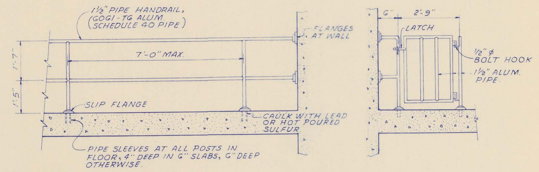
1 1/2" ALUMINUM PIPE HANDRAIL N.T.S.
