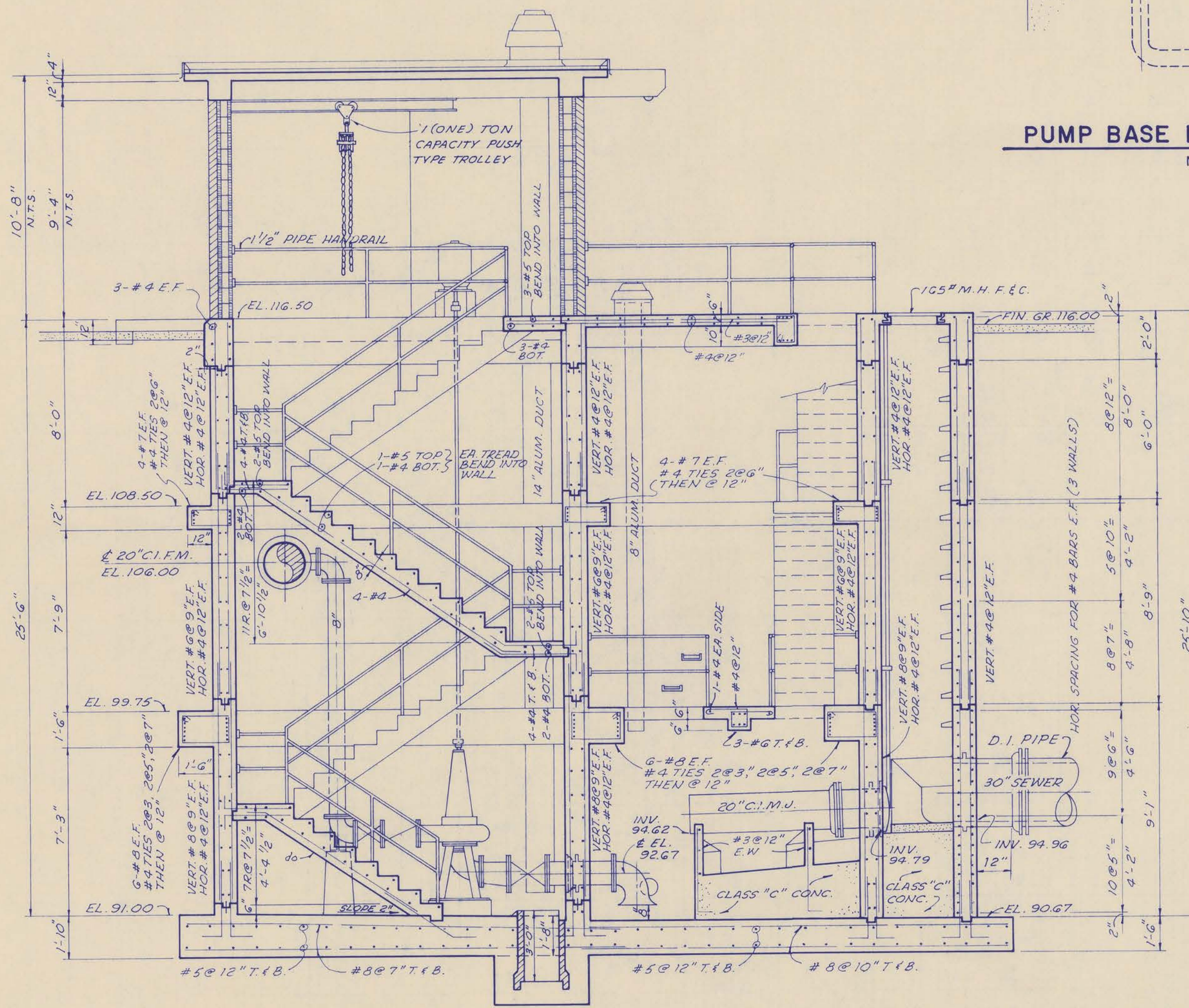
SECTION C-C 1/4"=1'-0"
