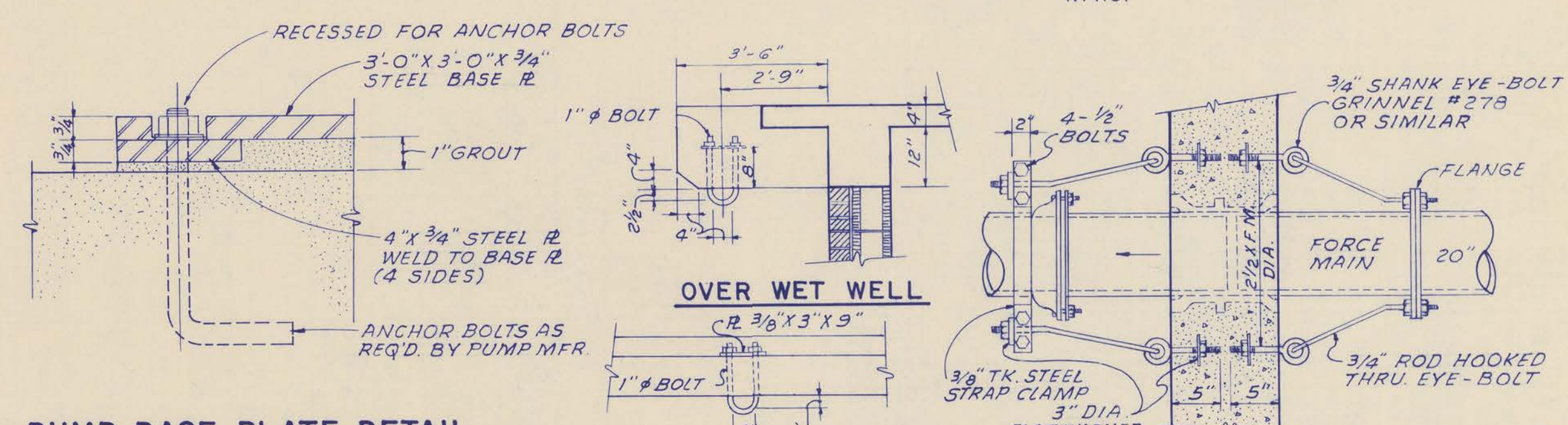
PUMP BASE PLATE DETAIL N.T.S.
