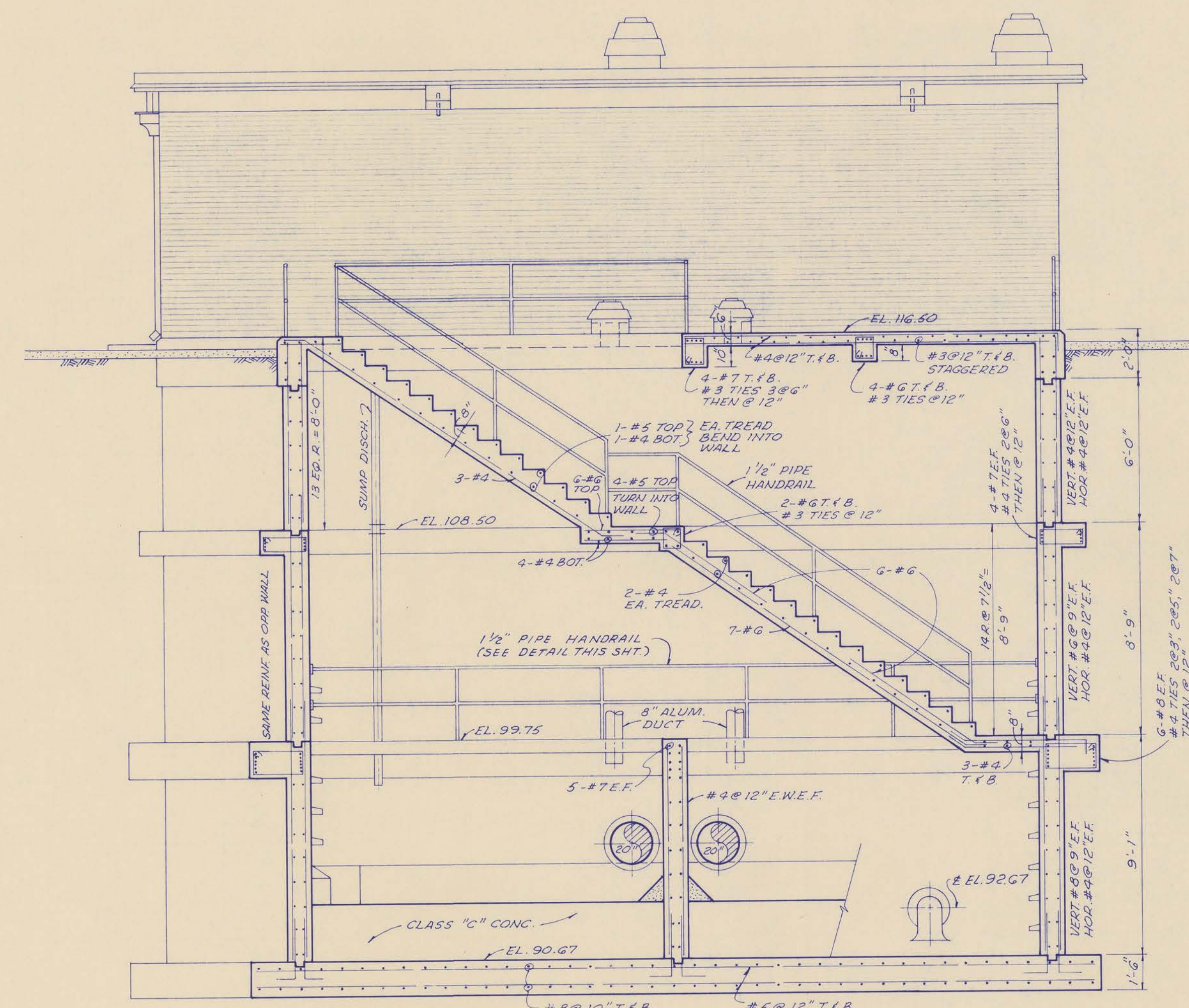
SECTION B-B 1/4"=1'-0"
