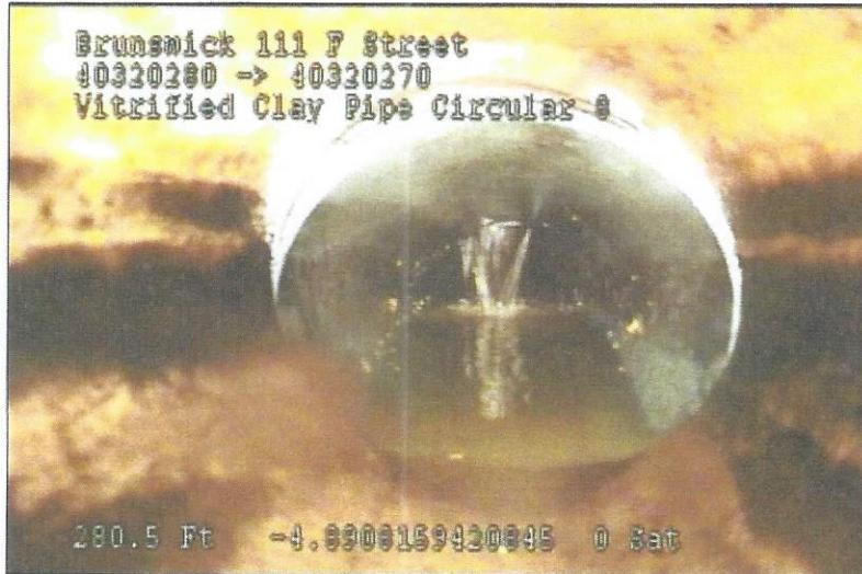
Photo: 40320280_40320270_02052018_134435_A.jpg, VCR No.: 1 281.9FT, Joint Offset Medium
