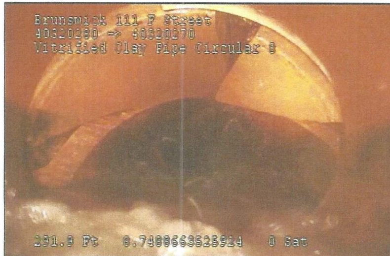
Photo: 40320280_40320270_30042018_104417_A.JPG, VCR No.: 1 292.2FT, Broken Soil Visible, from 08 to 08 o'clock, within 8 inches of joint: YES
